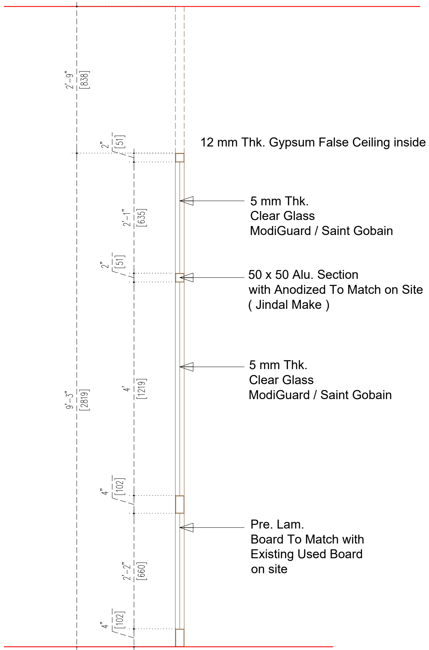
Anodized Alu. Partition Typical SECTION ( Anodized To match as on site )
