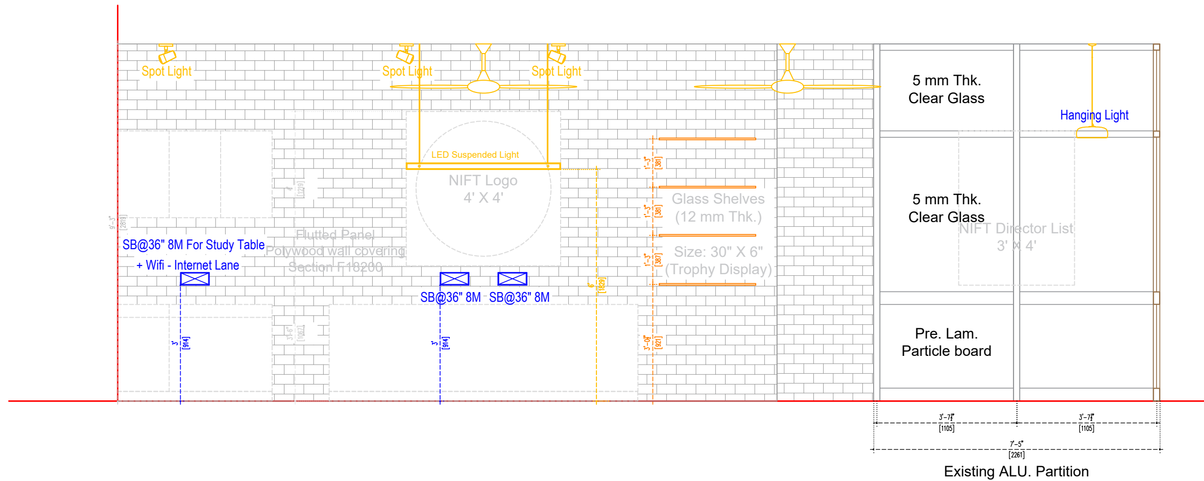
ELEVATION WALL- A
