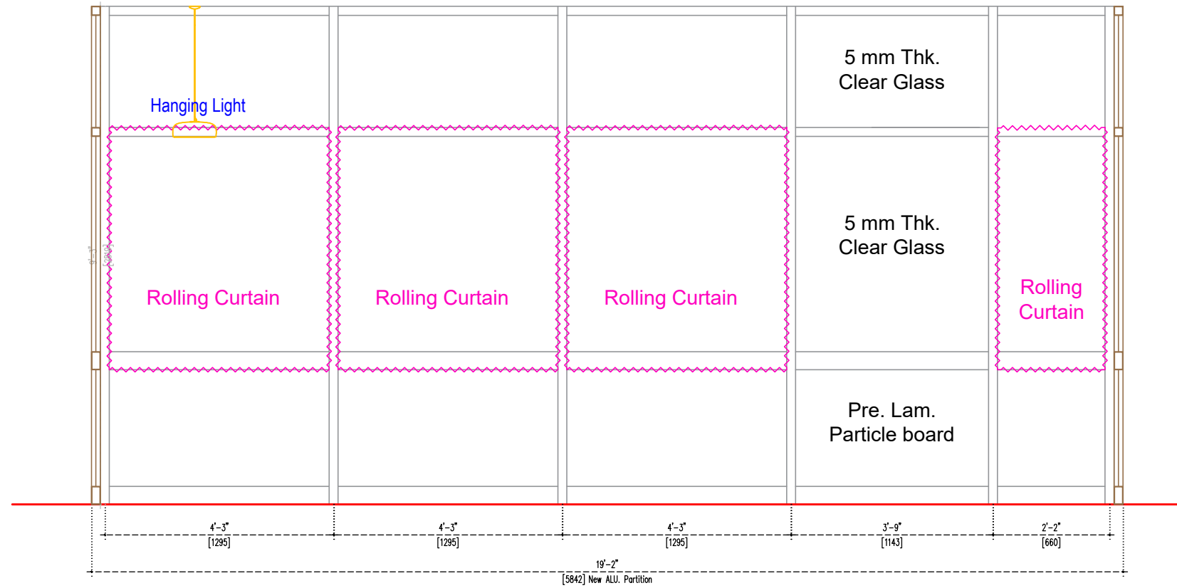
ELEVATION WALL-- B
