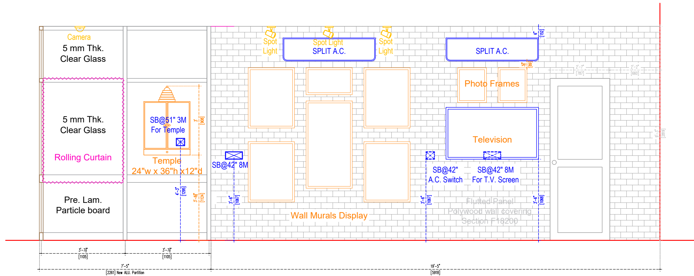
ELEVATION WALL- C
