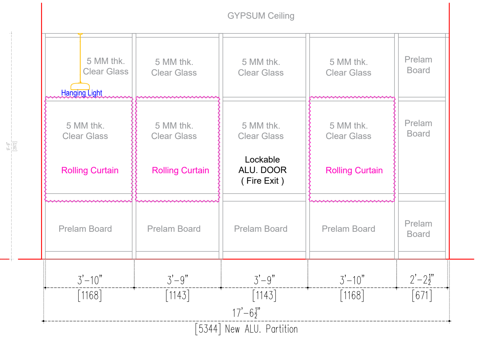
ELEVATION WALL- F
