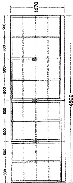
FRONT ELEVATION WITH DIMENSIONS
